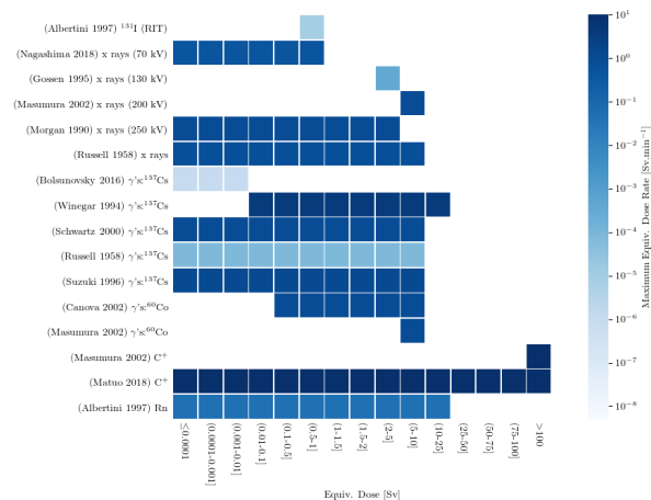
Figure 1: Plot of studies (y-axis) against equivalent dose (Sv) used to determine the empirical link between direct deposition of energy and increased cell mutation rates. The z-axis denotes the equivalent dose rate used in each study. The y-axis is ordered from low LET to high LET from top to bottom.
