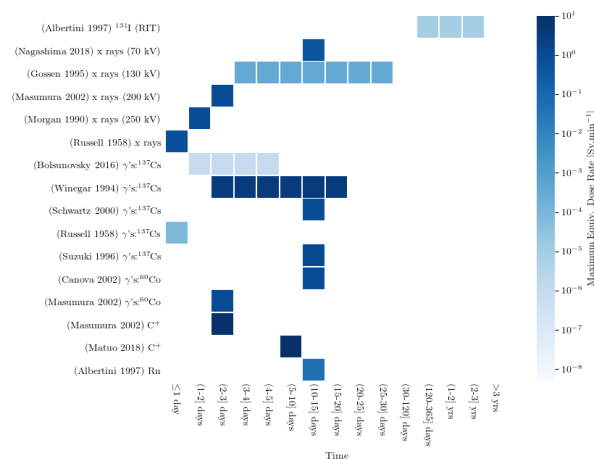
Figure 2: Plot of studies (y-axis) against time scales used to determine the empirical link between direct deposition of energy and increased cell mutation rates. The z-axis denotes the equivalent dose rate used in each study. The y-axis is ordered from low LET to high LET from top to bottom.
