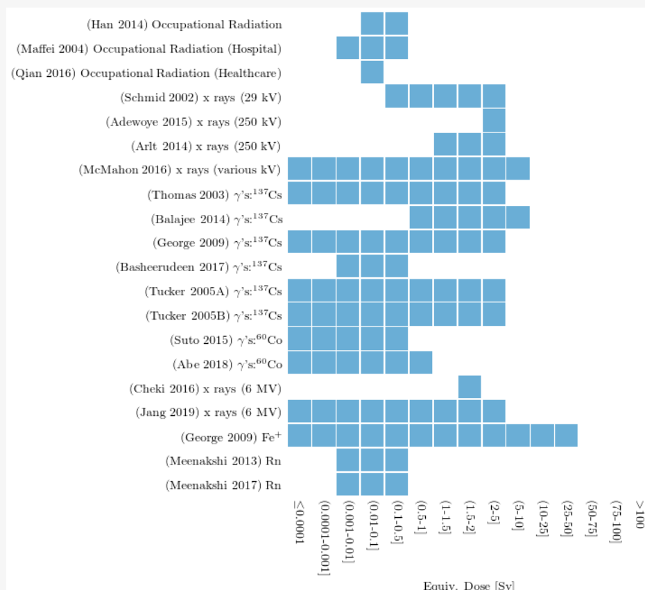
Figure 1: Plot of example studies (y-axis) against equivalent dose (Sv) used to determine the empirical link between direct deposition of energy and increased rates of chromosomal aberrations. The y-axis is ordered from low LET to high LET from top to bottom.
