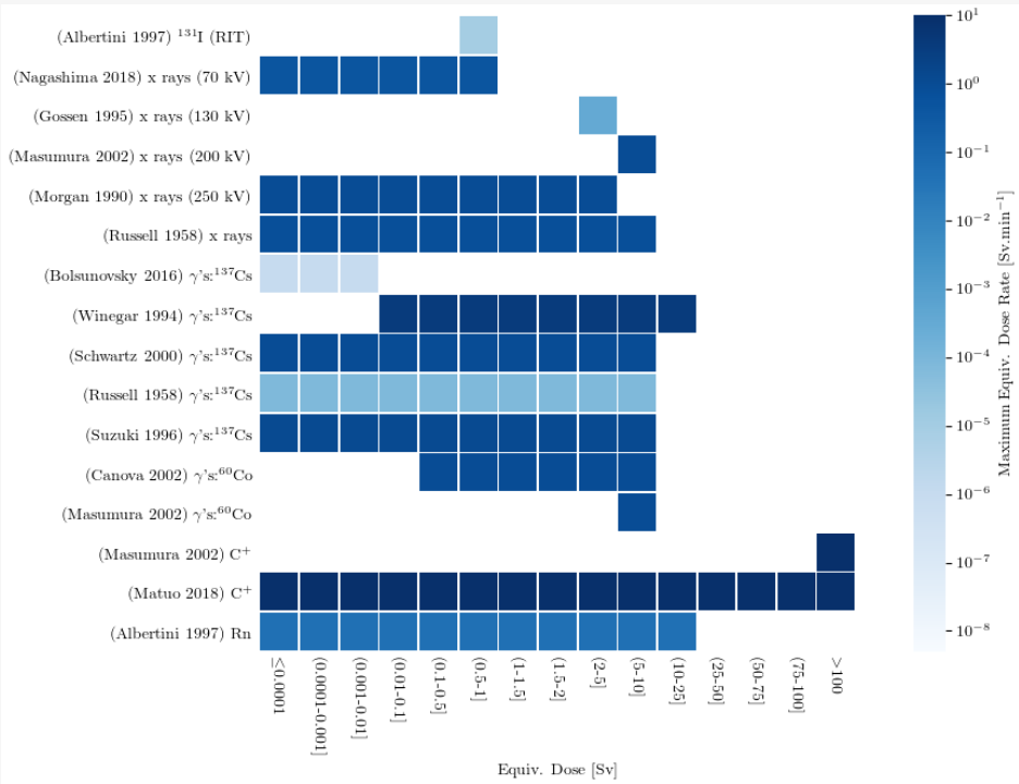
Figure 1: Plot of example studies (y-axis) against equivalent dose (Sv) used to determine the empirical link between direct deposition of energy and increased cell mutation rates. The z-axis denotes the equivalent dose rate used in each study. The y-axis is ordered from low LET to high LET from top to bottom.
